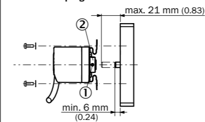
Figure 1: Installing the DBS36 blind hollow shaft with stator coupling
