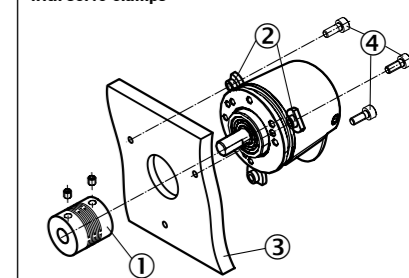
Figure 5: Installing the DBS36 face mount flange with servo-clamps
