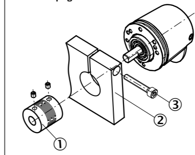
Figure 4: Installing the DBS36 face mount flange via the clamping attachment
