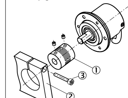
Figure 7: Installing the DBS50 face mount flange via the clamping attachment
